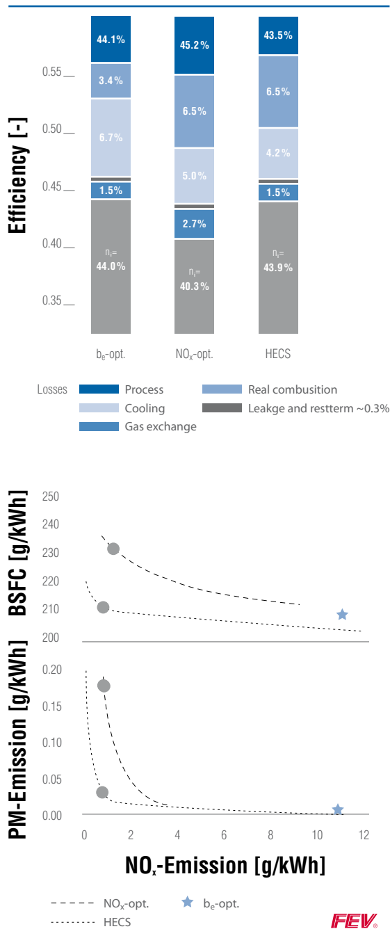
Fig. 1: Emission Performance and Efficiency of the HECS Engine (Part Load Point @ ~2300 rpm)
